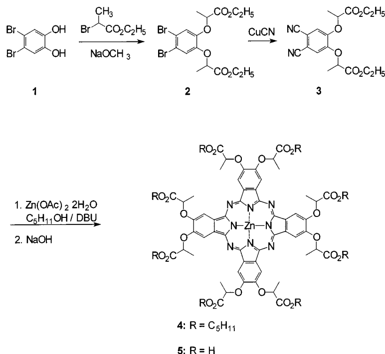
Scheme 1. Synthesis of phthalocyanine 5 starting from 4,5-dibromocatechol ( 1 )
