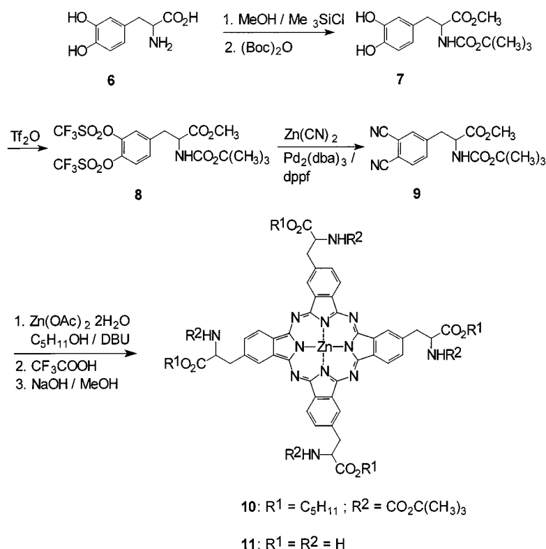
Scheme 2. Synthetic route to phthalocyaninato zinc amino acid 11
