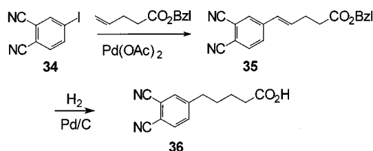
Scheme 6. Synthesis of 36
