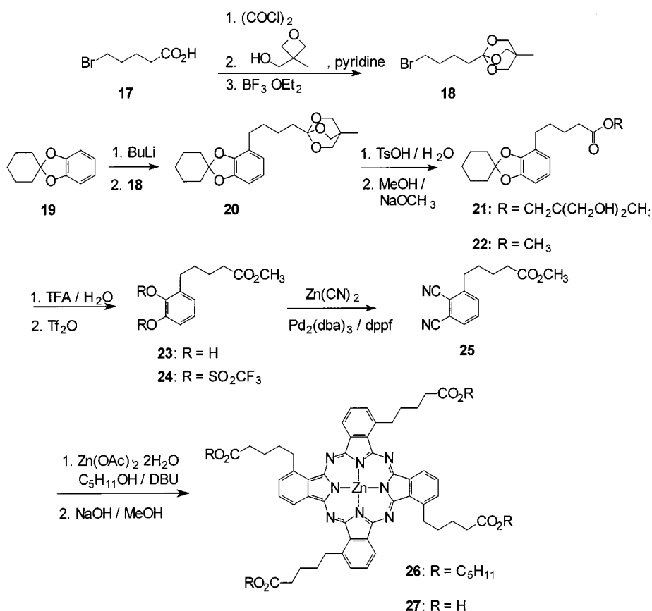
Scheme 4. Synthesis of 27 starting from the protected catechol 19
