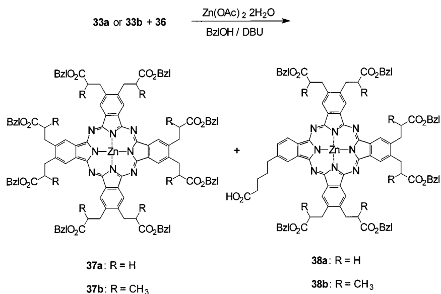
Scheme 7. Statistical condensation of 33 and 36
