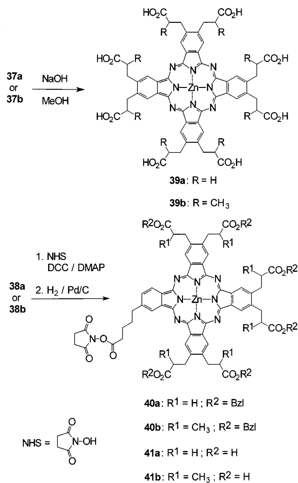
Scheme 8. Synthesis of the phthalocyanines 39 , 40 and 41
