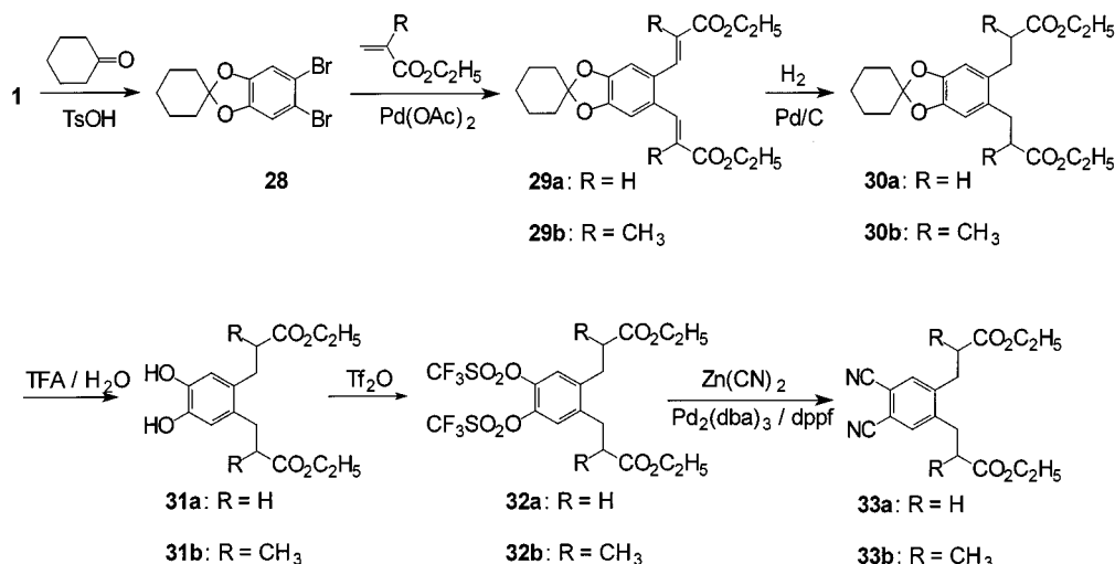
Scheme 5. Synthesis of the phthalonitriles 33a and 33b
