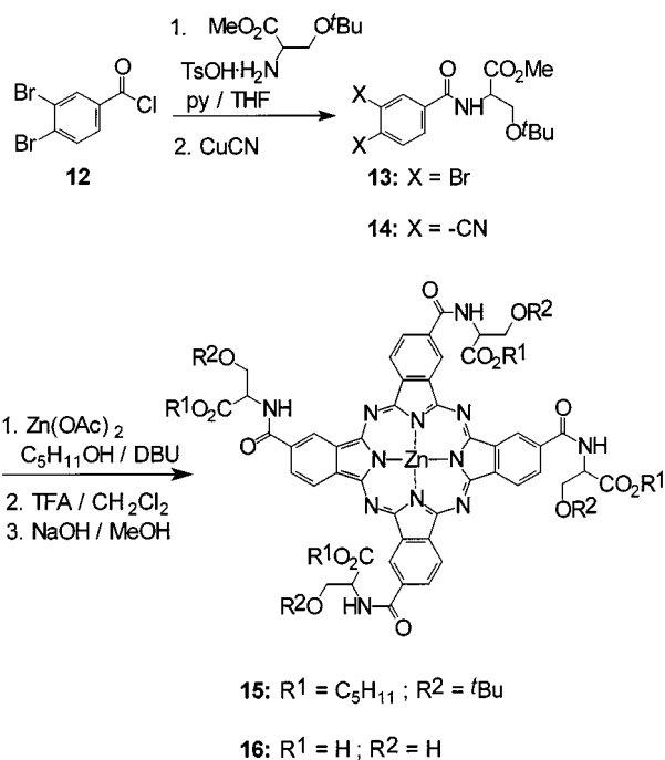
Scheme 3. Synthesis of phthalocyanine 16
